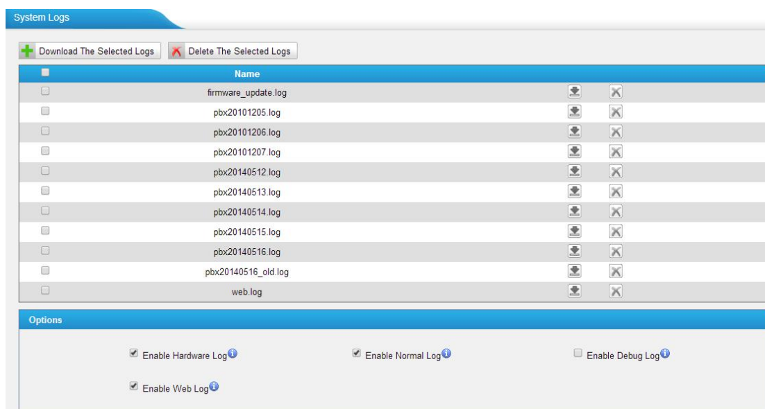
Figure 13-2 System Logs
