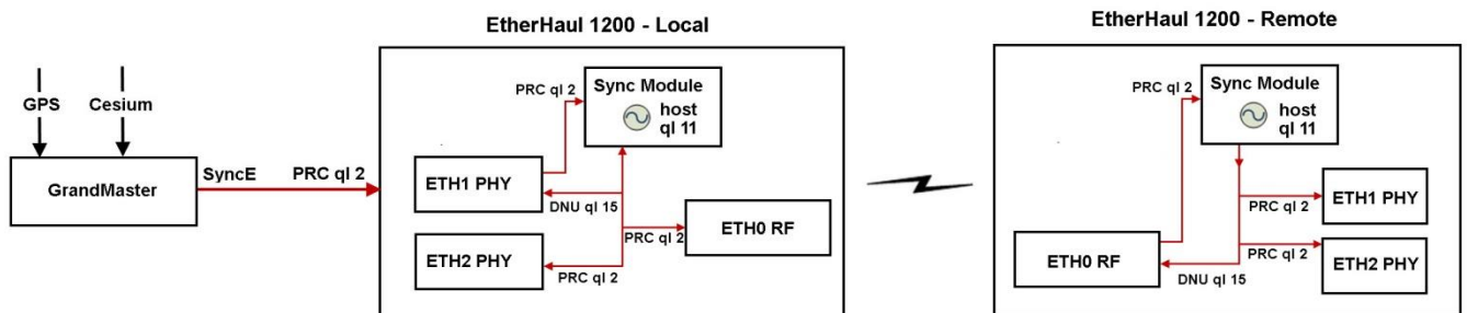
Figure 10-3 Typical SyncE Scenario – Normal Operation
