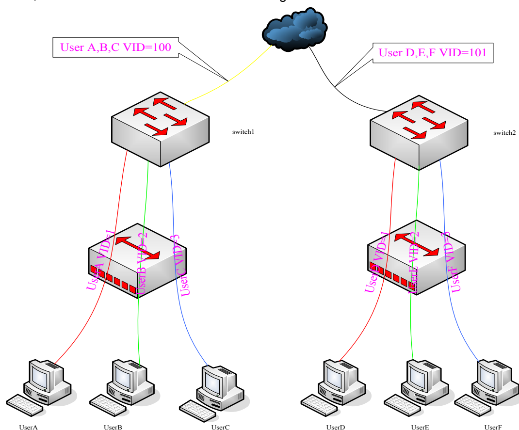
Fig 1-11 VLAN-translation typical application
