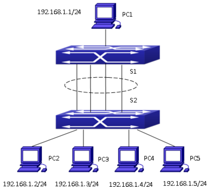
Fig 6-4 Load Balance
