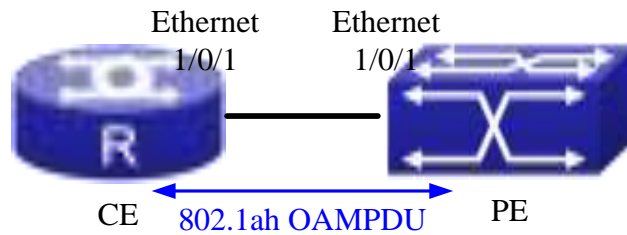
Fig 10-3 Typical OAM application topology
