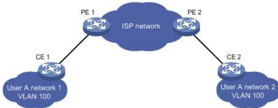
Fig 12-2 BPDU Tunnel application environment
