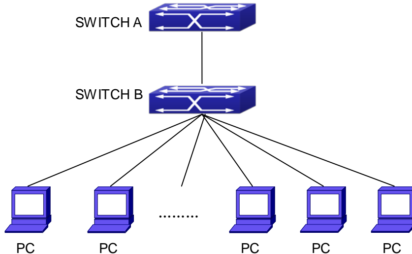
Fig 4-1 The Number Limitation of MAC in Port Typical Configuration Example
