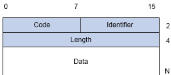
Fig 3-4 the Format of EAP Data Packets
