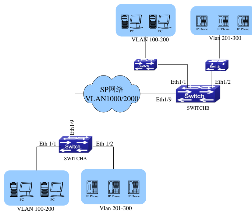
Fig 1-5 Selective QinQ application
