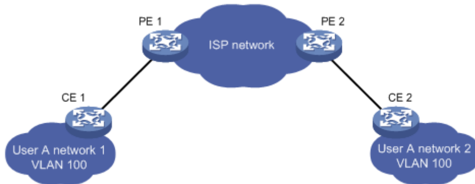
Fig 12-2 BPDU Tunnel application environment
