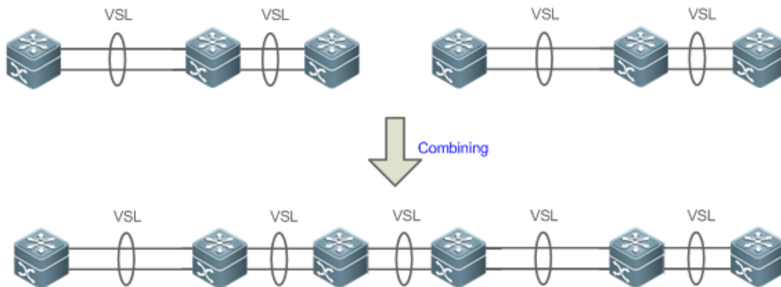
Figure 8-12 Topology combining
