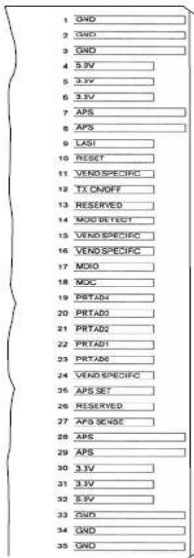
Top view -Top side of PCB
