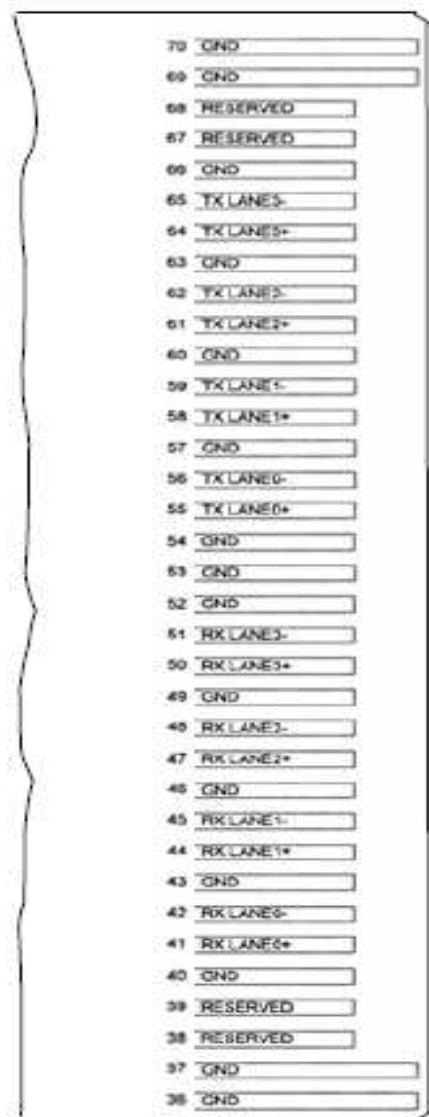
Top view-Bottom side of PCB
