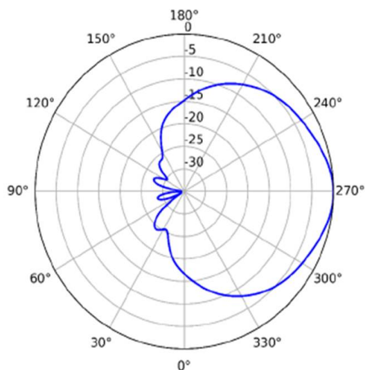
2.4GHz (Horizontal)
