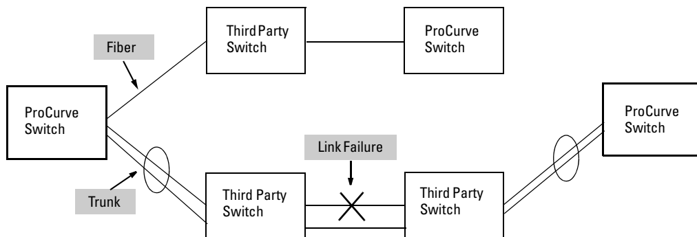
Figure 10-20. UDLD Example
