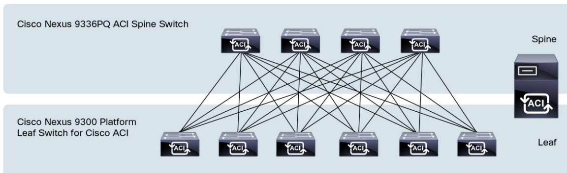
Figure 10. Cisco Nexus 9300 Platform Leaf-and-Spine Architecture for Cisco ACI
