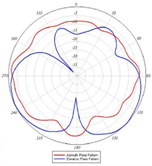
5-GHz Element 2 Azimuth and Elevation Plane Patterns
