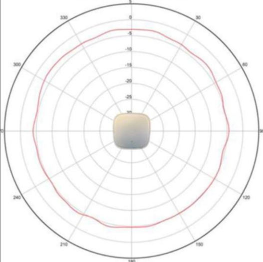
5 GHz Azimuth
