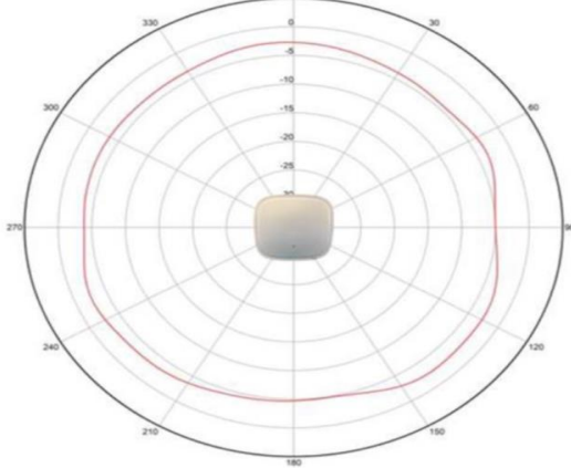
2.4 GHz Azimuth
