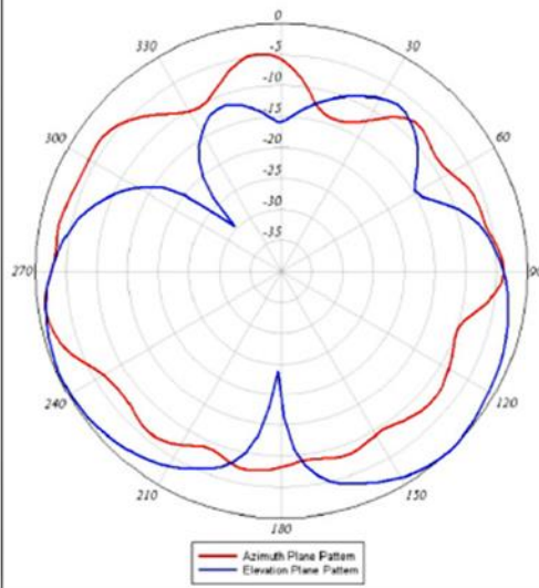
5-GHz Element 3 Azimuth and Elevation Plane Patterns
