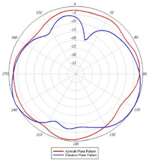
2.4-GHz Element 3 Azimuth and Elevation Plane Patterns
