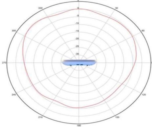
2.4 GHz Elevation
