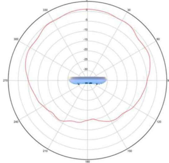
5 GHz Elevation
