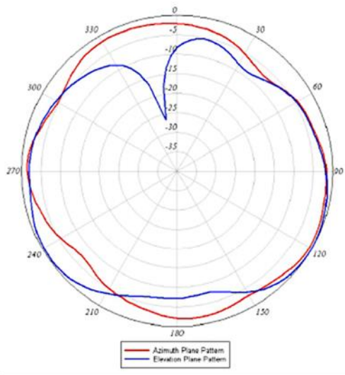
2.4-GHz Element 2 Azimuth and Elevation Plane Patterns
