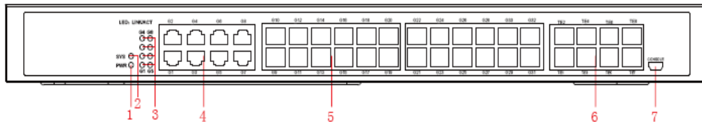
Figure 1-1 Front template of the S3940F switch
