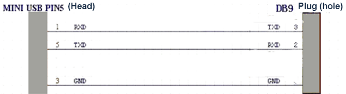
Figure 3-4 Cable connection at the console port
