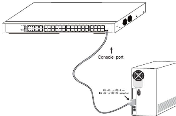
Figure 3-5 Connecting the console port of S3940F and computer
