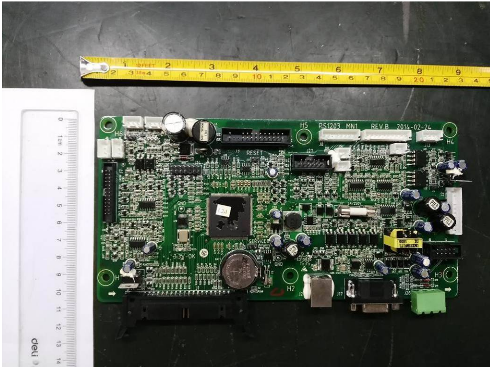
Fig. 12 –PCB view
