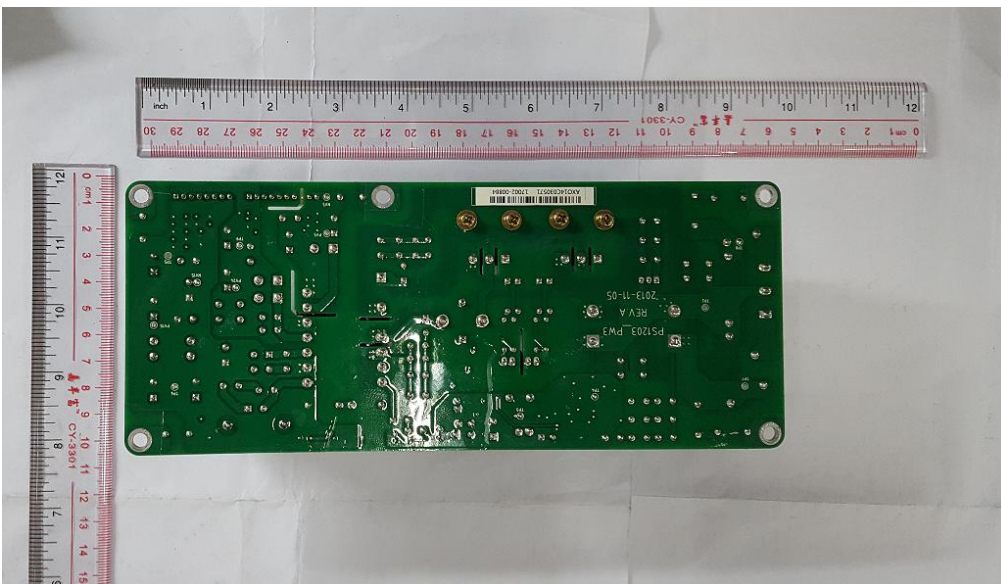
Fig. 15 – PCB view
