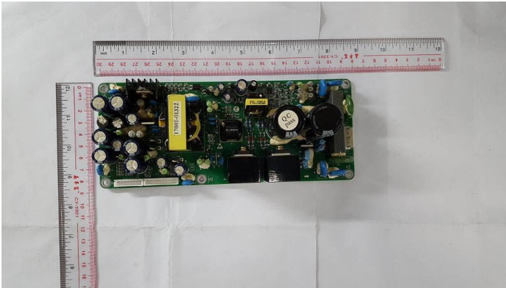
Fig. 14 –PCB view
