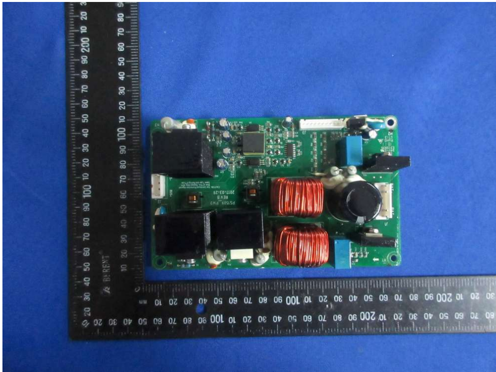
Figure 17: PCB component view
