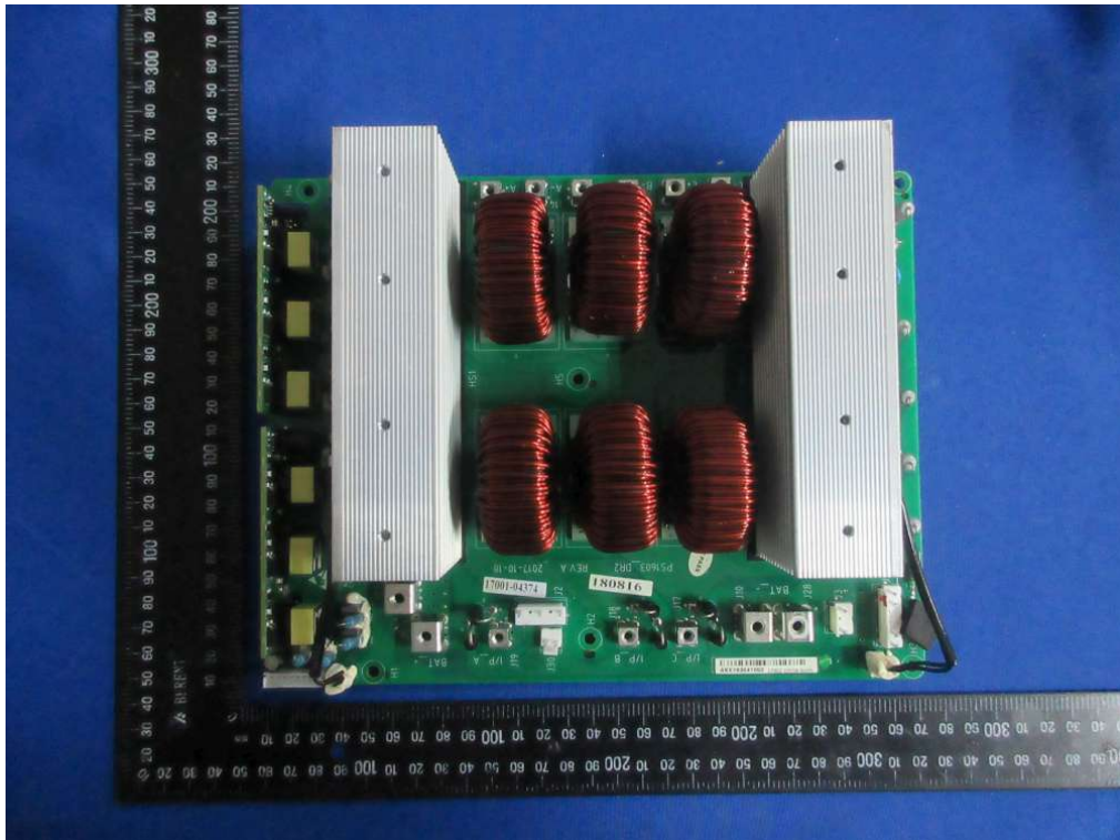
Figure 13: PCB component view
