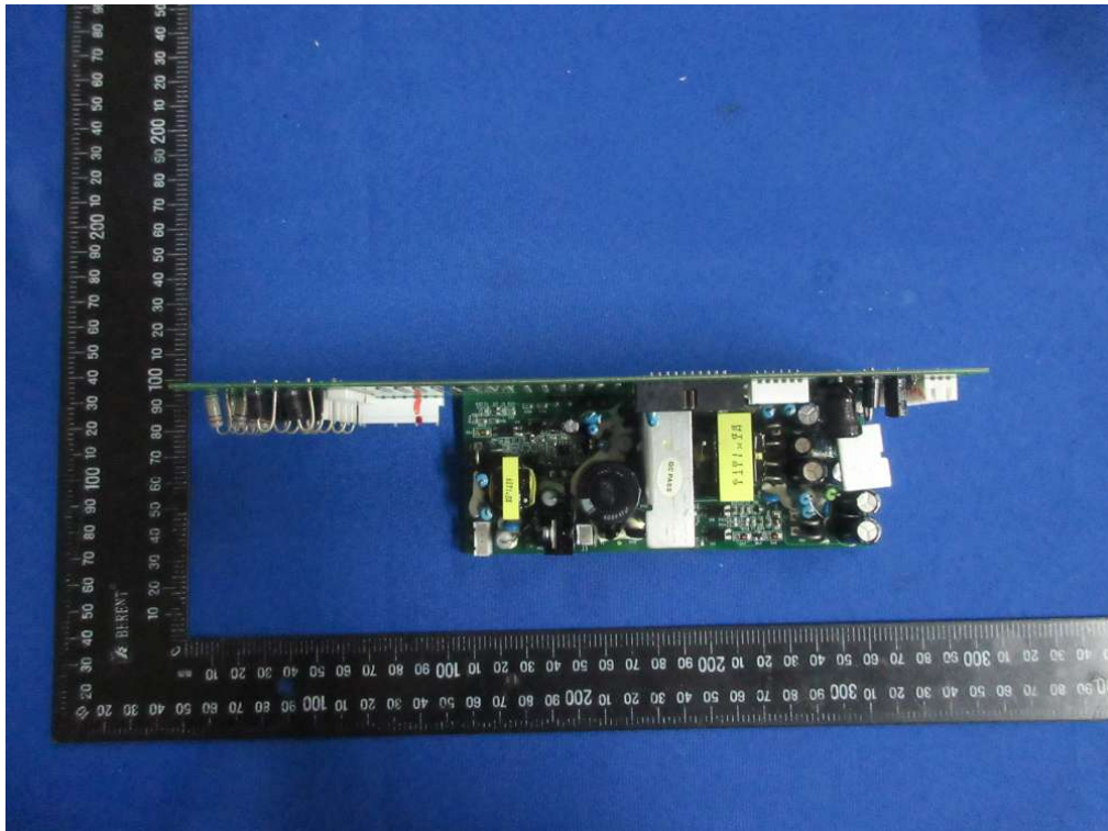
Figure 9: PCB component view
