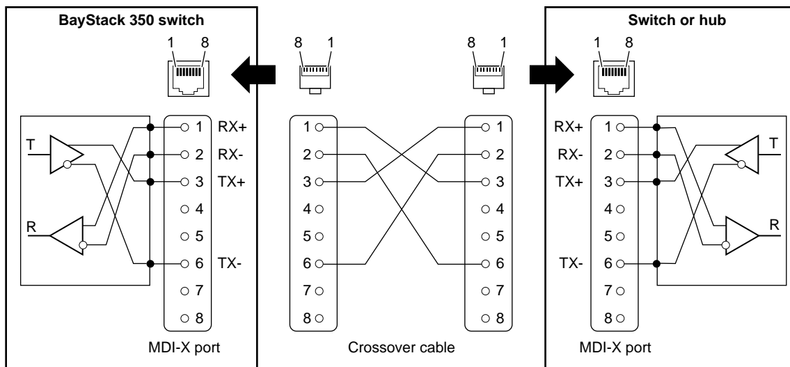
Figure E-3. MDI-X to MDI-X Cable Connections
