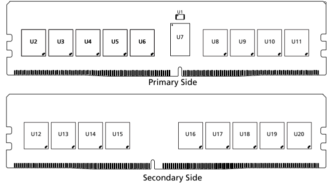
Figure 1: 288-Pin RDIMM (MO-309, R/C-E3)
