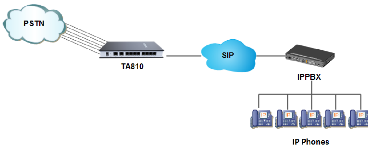
Figure 2-2 Connect IPPBX and TA FXO Gateway
