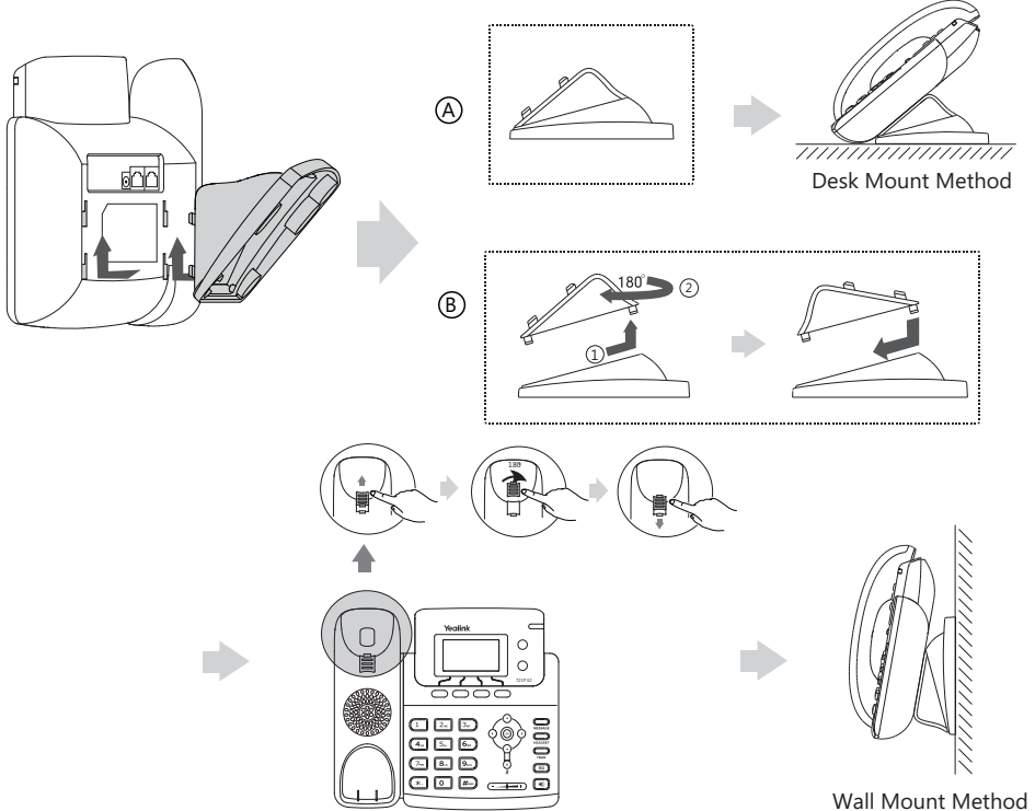
Wall Mount Method
