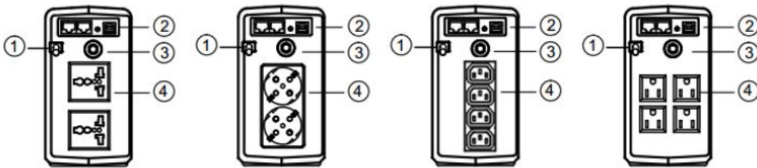
Rear panel of 400 VA – 800 VA UPS
