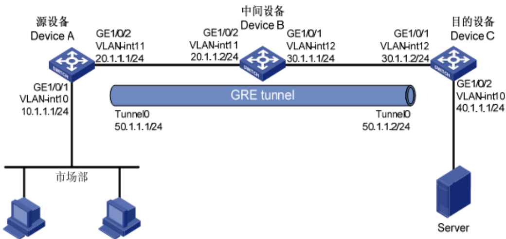
Fig 4-1 ERSPAN application diagram
