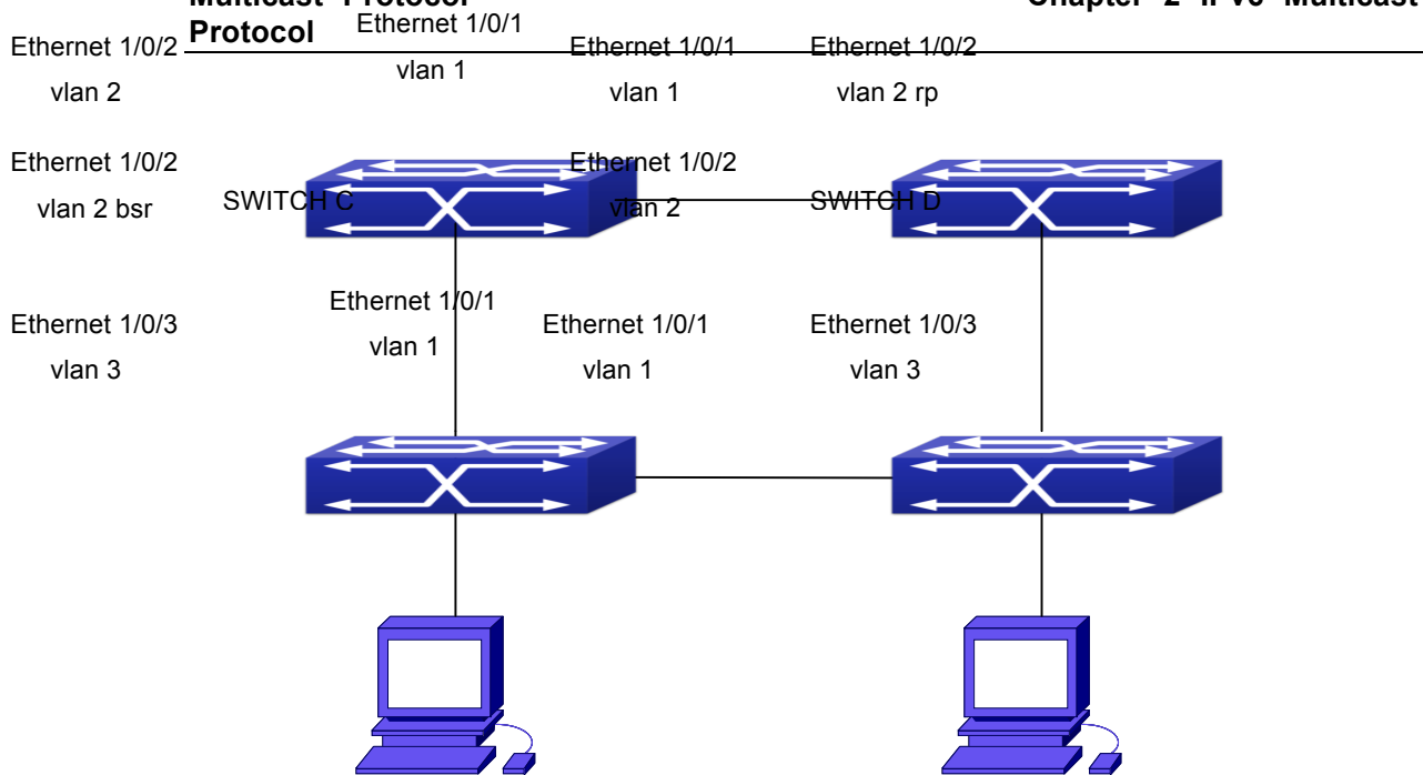
Fig 2-4 PIM-SSM typical environment
