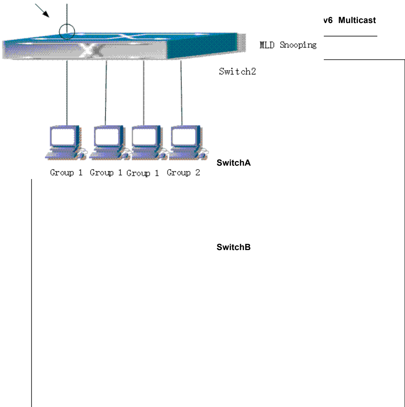
Fig 2-7 Switch as MLD Querier Function figure
