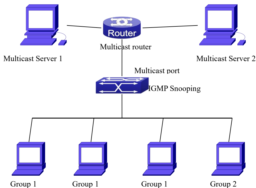
Figure 4-2 Enabling IGMP Snooping function
