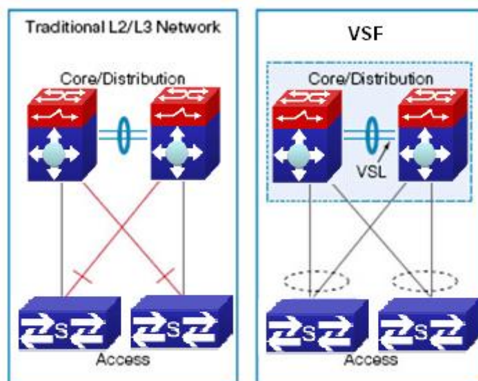
Figure 9-2 VSF
