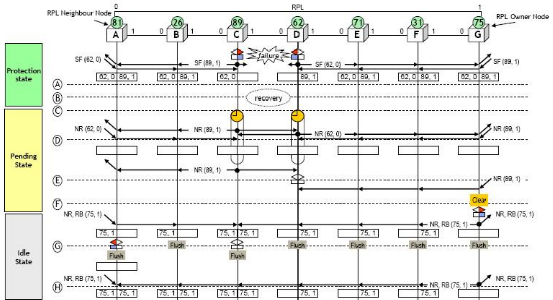
Figure 6-17 Non-revertive switch fault restoration of single link
