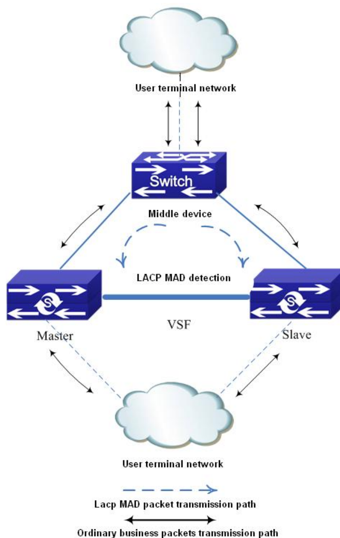
Figure 9-7 LACP MAD detection
