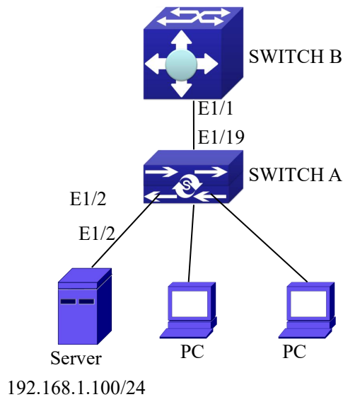
Figure 3- 1 ARP scanning prevention typical configuration example
