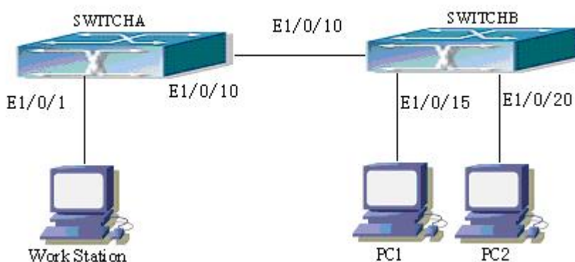
Figure 4-6 Function configuration of the Multicast VLAN
