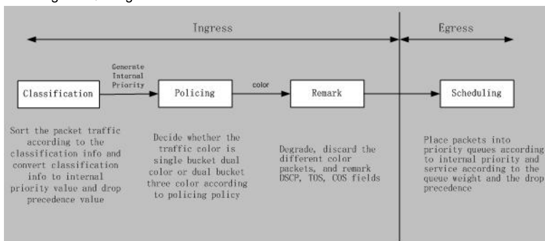
Figure 5-42 Basic QoS Model
