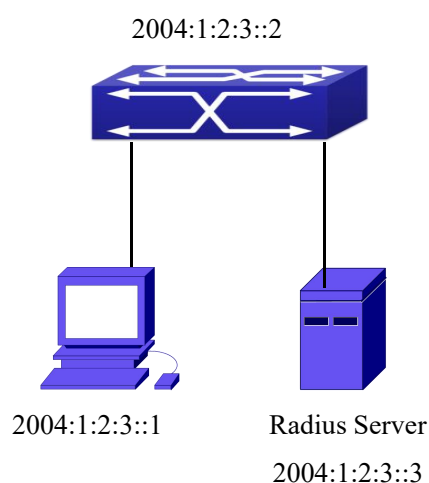
Figure 5- 17 IPv6 Radius
