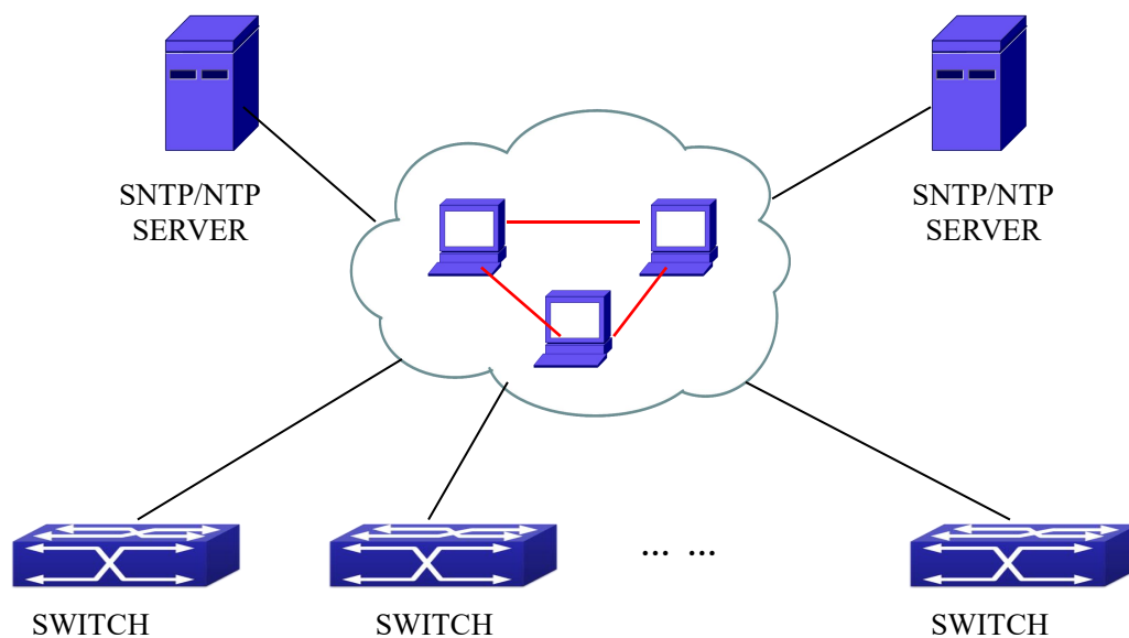
Figure 8-3 Typical SNTP Configuration
