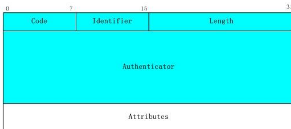
Figure 5- 20 Message structure for RADIUS
