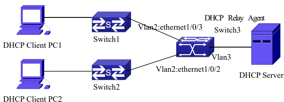
Figure 3-8 A DHCP option 82 typical application example
