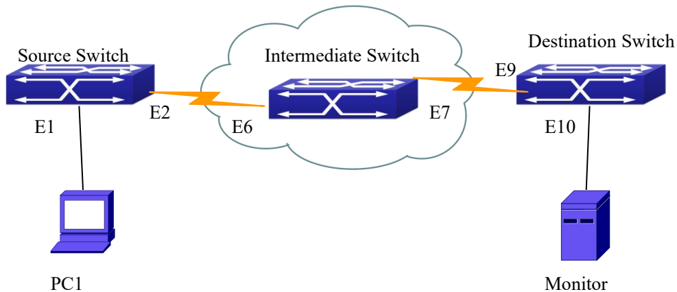
Figure 7- 1 RSPAN Application Sample
