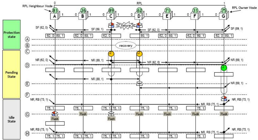
Figure 6-16 Revertive switch fault restoration of single link
