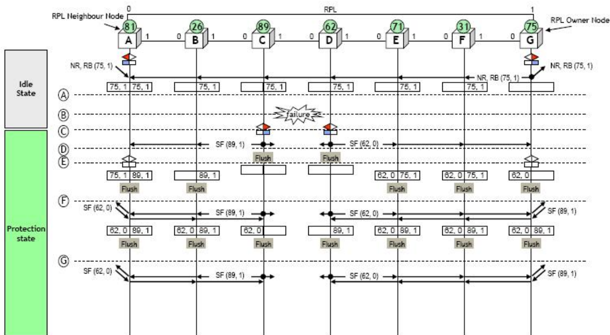
Figure 6- 15 single-link fault
