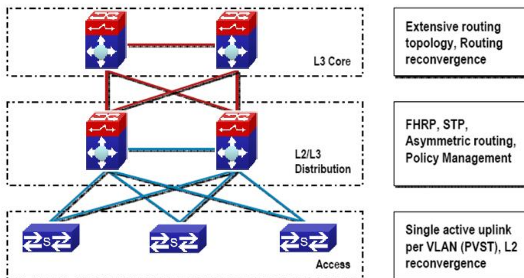
Figure 9- 1 Traditional Enterprise Network
