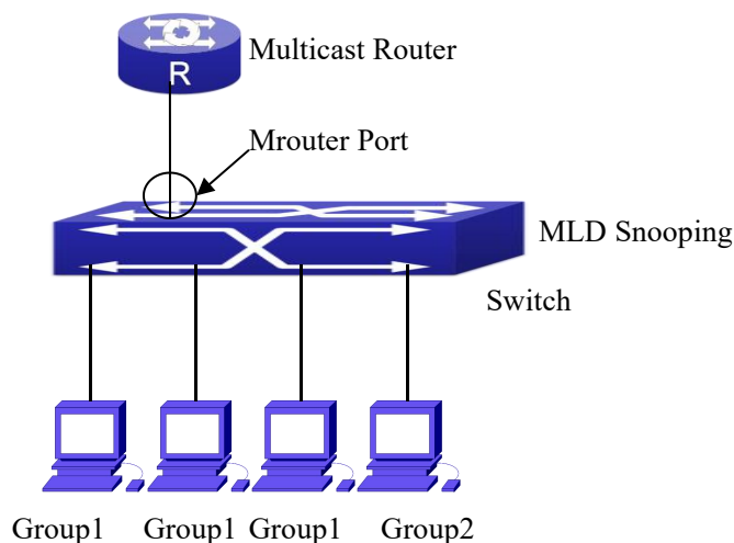
Figure 10-5 Open the switch MLD Snooping Function figure
