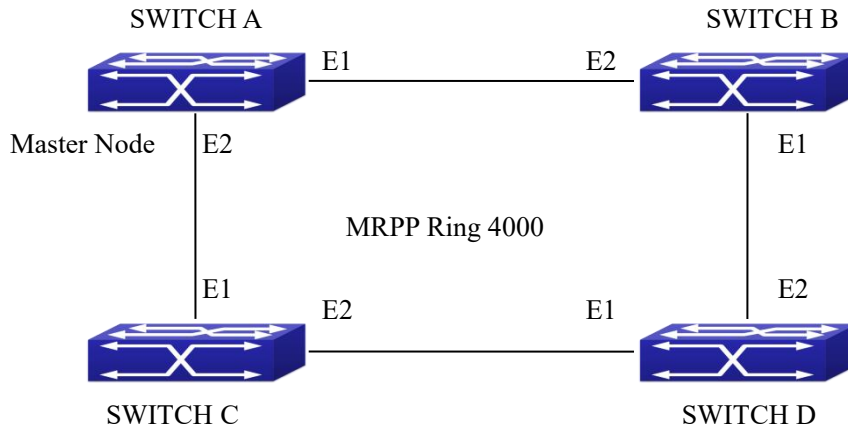
Figure 6-8 MRPP typical configuration scenario
