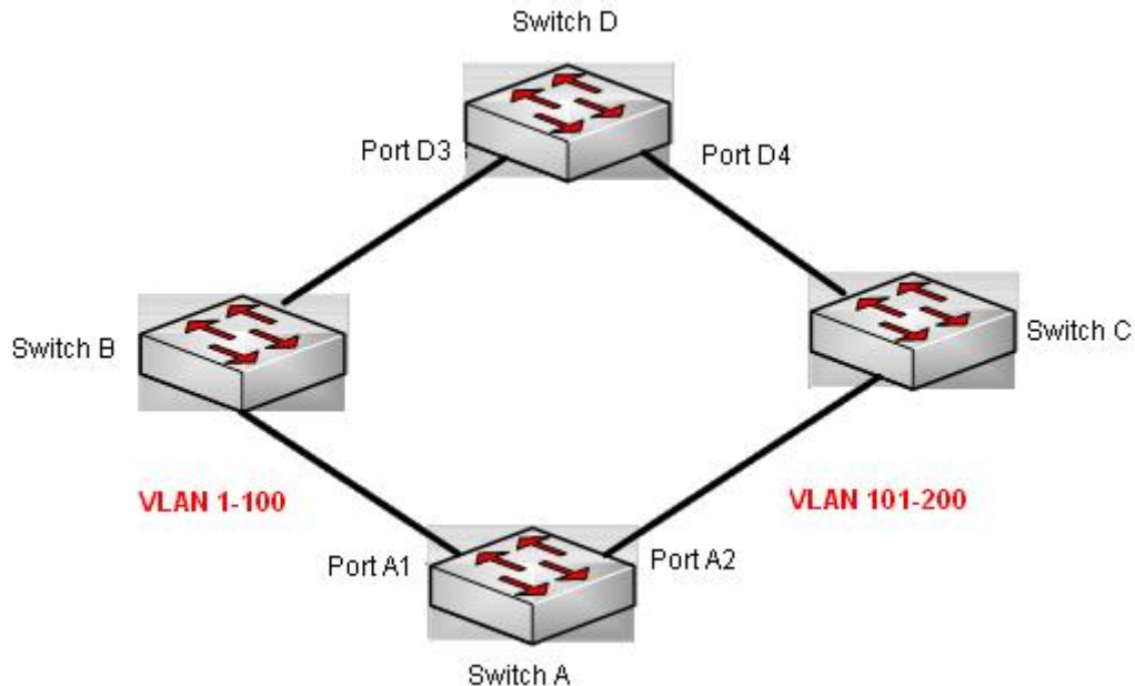
Figure 6- 10 VLAN load balance
