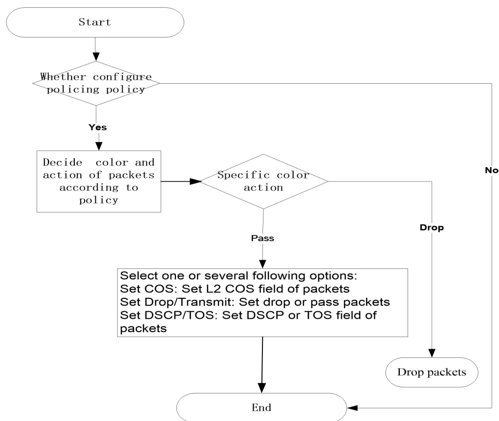
Figure 5-48 Egress QoS detail description
