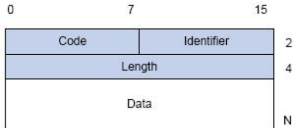
Figure 5-4 the Format of EAP Data Packets
