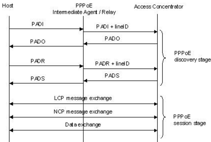
Figure 5- 36 PPPoE IA protocol exchange process
