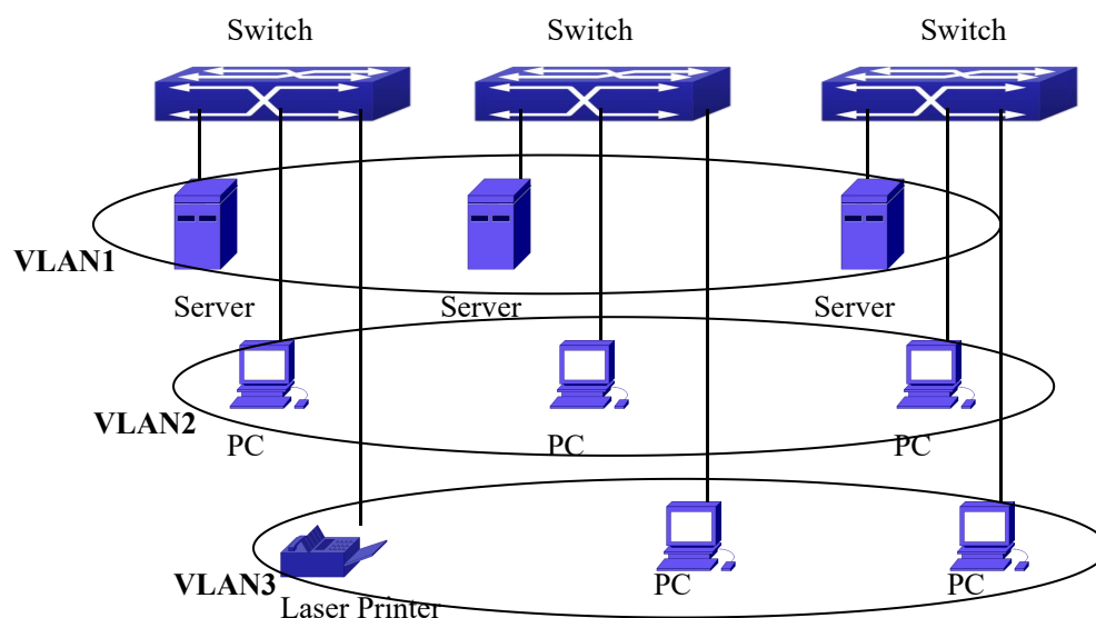
Figure 2- 18 VLAN network defined logically
