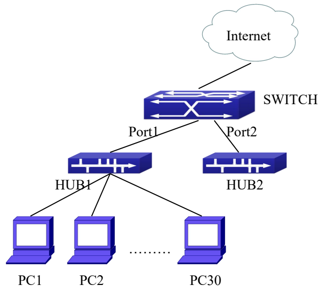
Figure 5- 18 a typical configuration example of AM function
