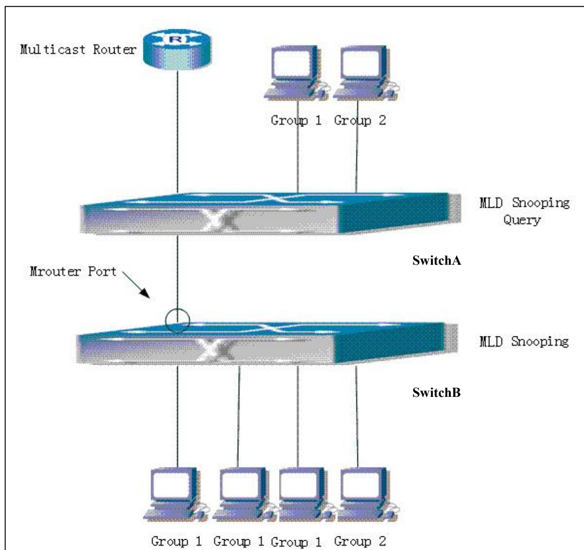
Figure 10-6 Switch as MLD Querier Function figure
