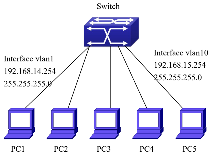
Figure 3-3 Gratuitous ARP Configuration Example
