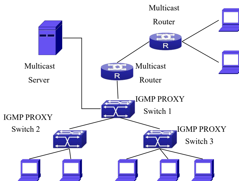
Figure 4-5 IGMP Proxy for multicast sources from downstream ports
