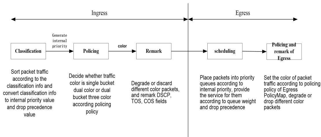
Figure 5-47 Basic Egress QoS Model
