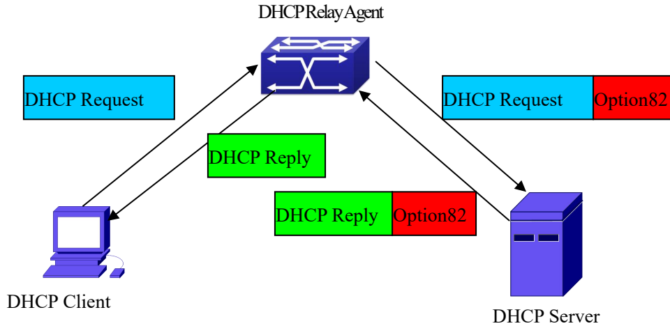
Figure 3- 7 DHCP option 82 flow chart
