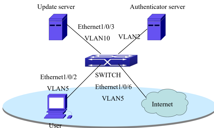
Figure 5- 15 User Being Online, VLAN Being Offline
