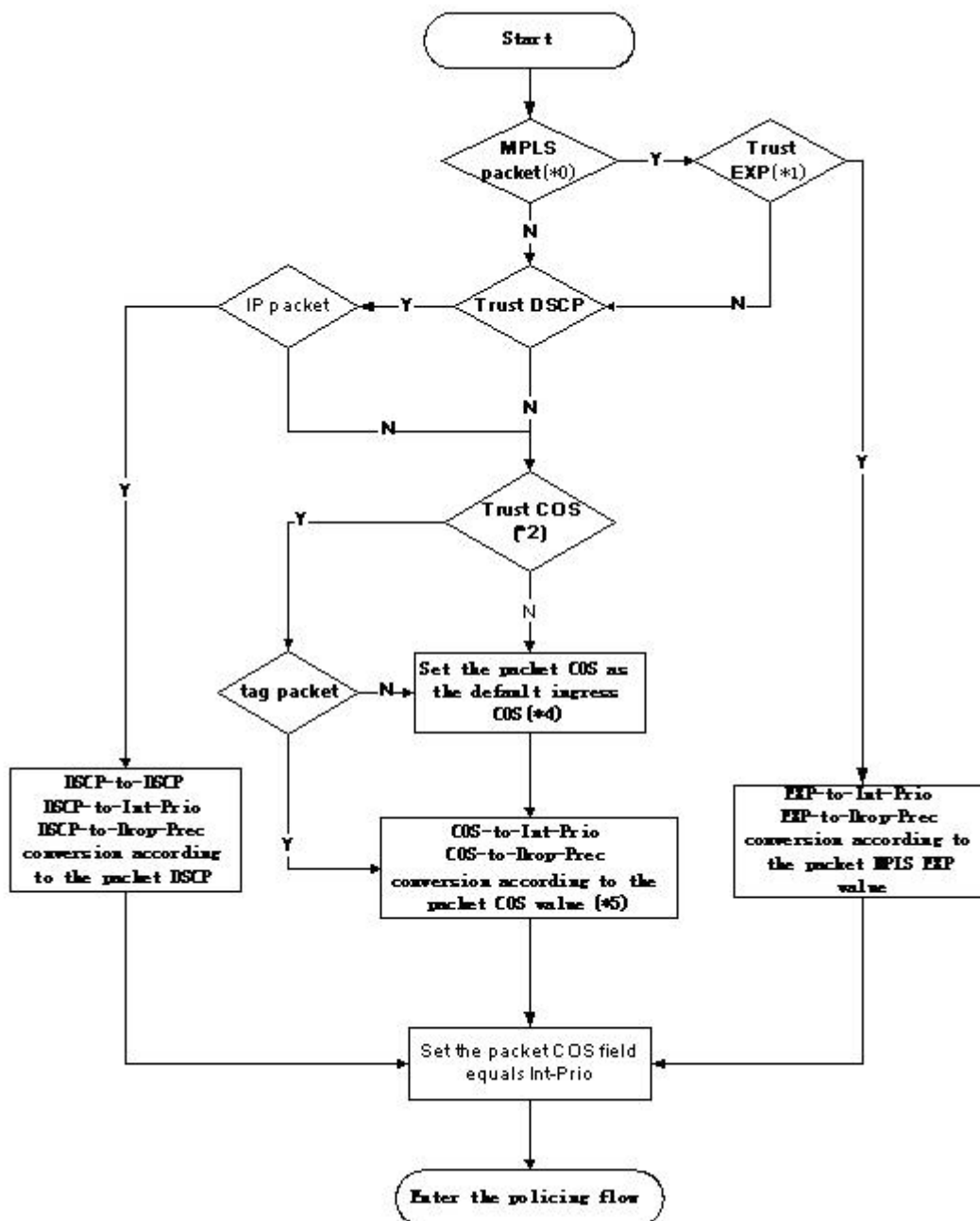
Figure 5-43 Classification process
