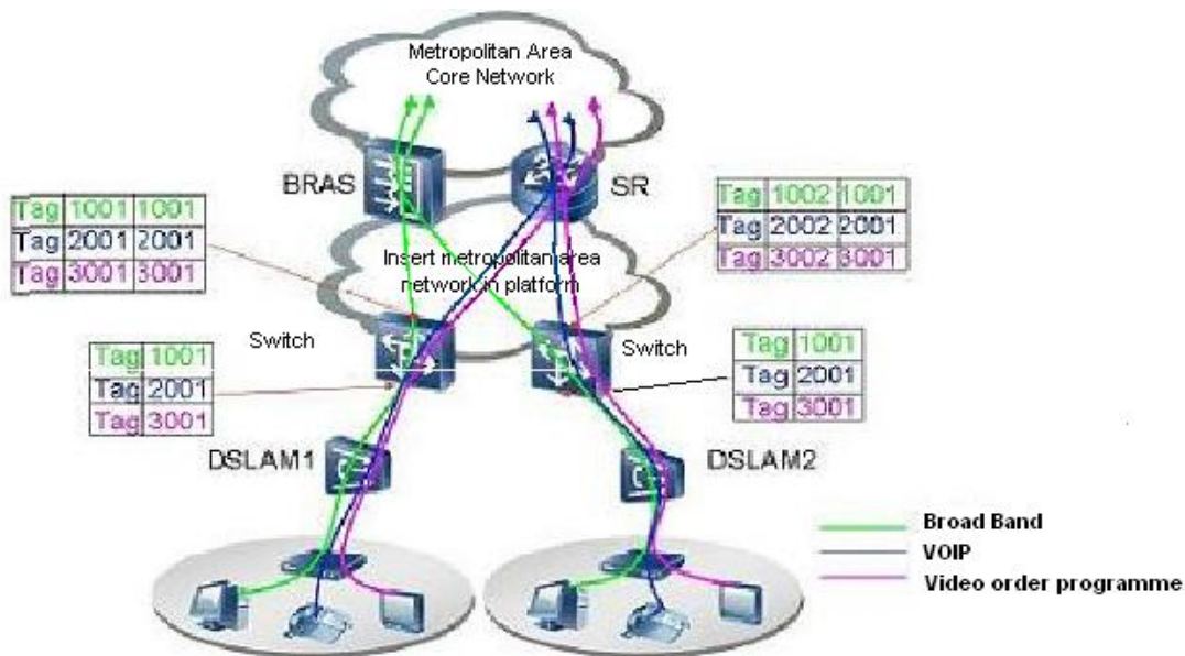
Figure 5-49 Flexible QinQ application topology
