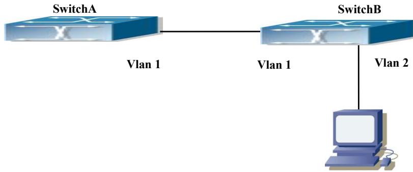
Figure 10-4 Network Topology Diagram
