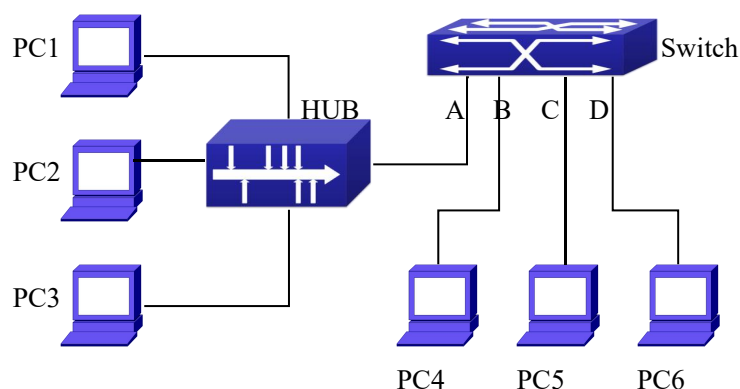
Figure 3-2 ARP GUARD schematic diagram
