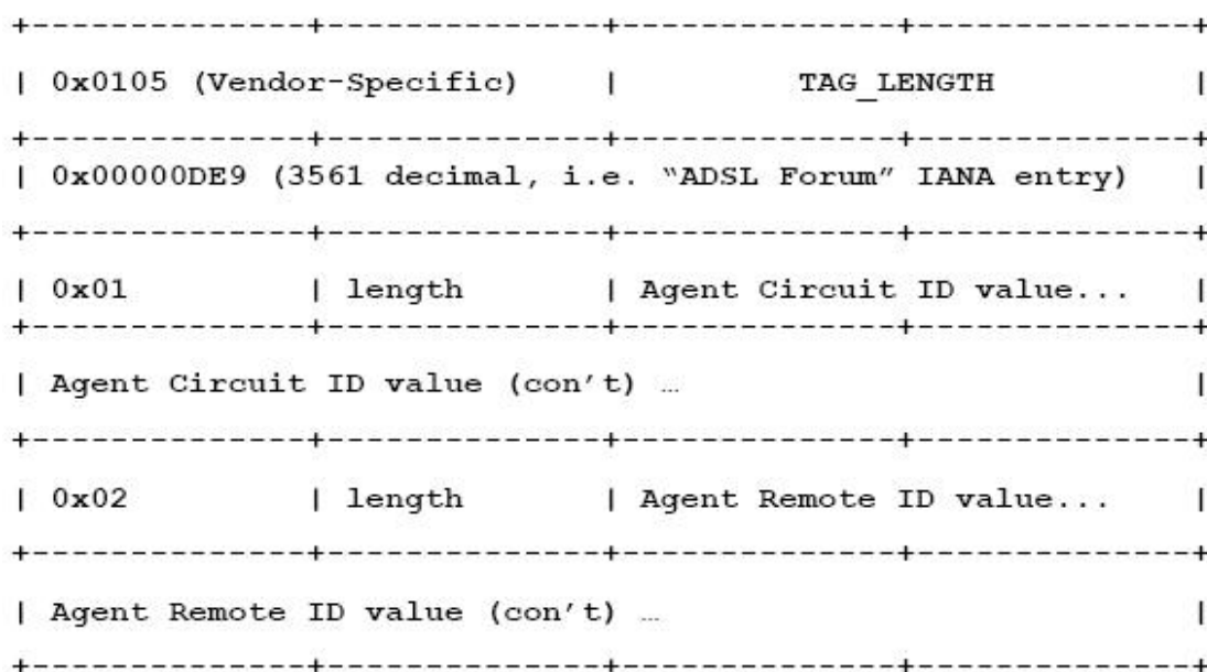
Figure 5-37 PPPoE IA - vendor tag (4 bytes in each row)
