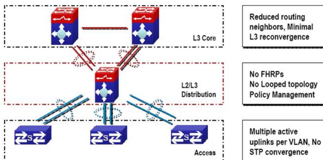
Figure 9-3 Enterprise that adopting virtual technology
