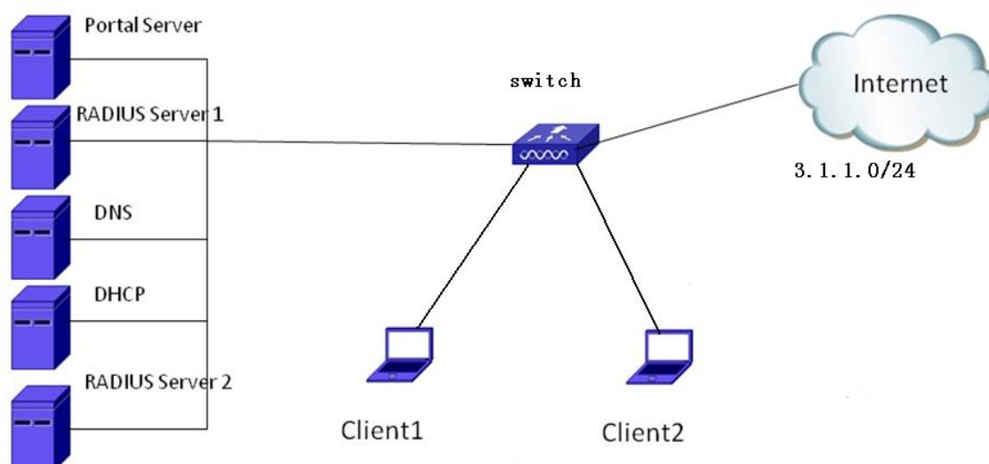
Figure 5-28 multi-portal servers function configuration
