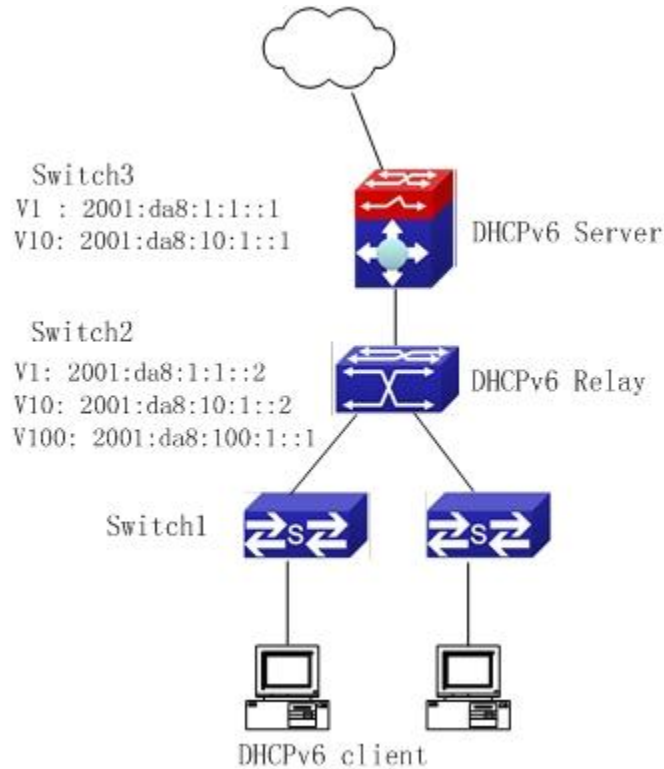
Figure 10-5 DHCPv6 relay option schematic
