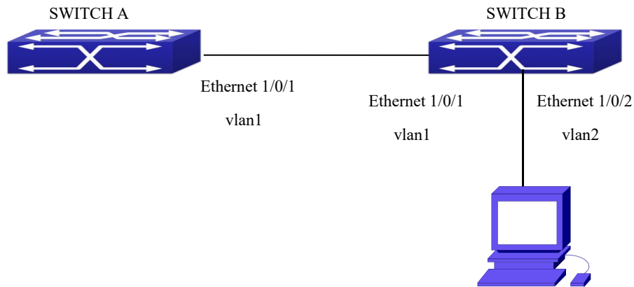
Figure 4- 1 IGMP Network Topology Diagram
