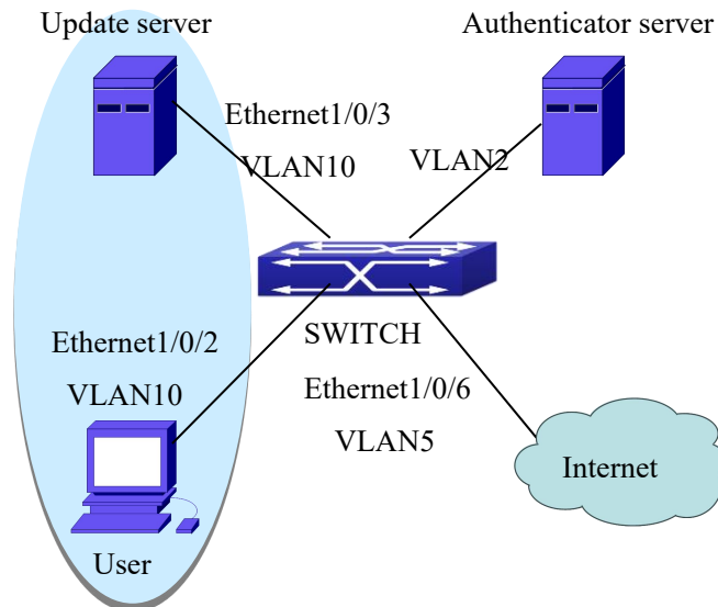
Figure 5-14 User Joining Guest VLAN
