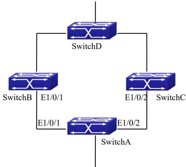
Figure 6- 11 ULPP typical example1
