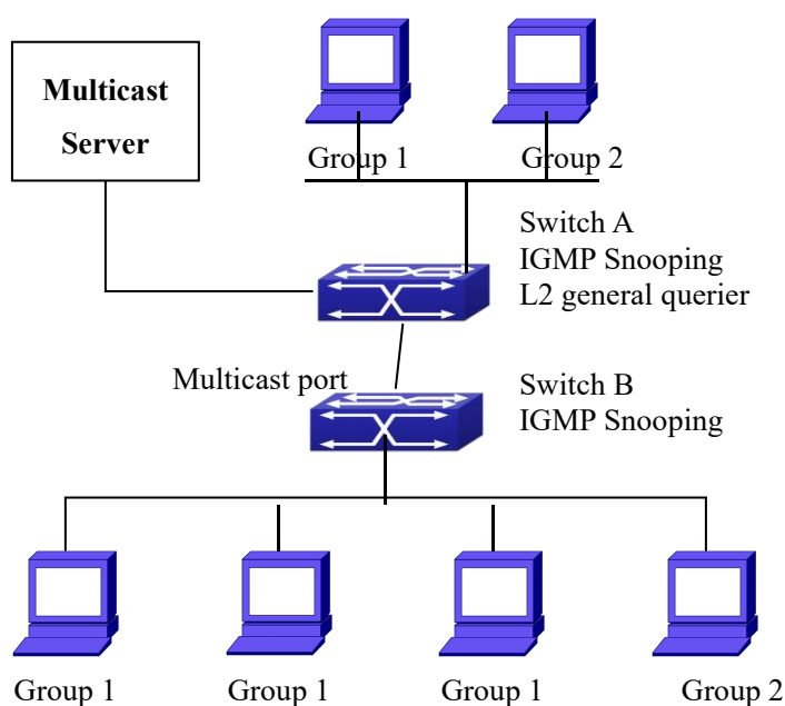
Figure 4-3 The switches as IGMP Queries
