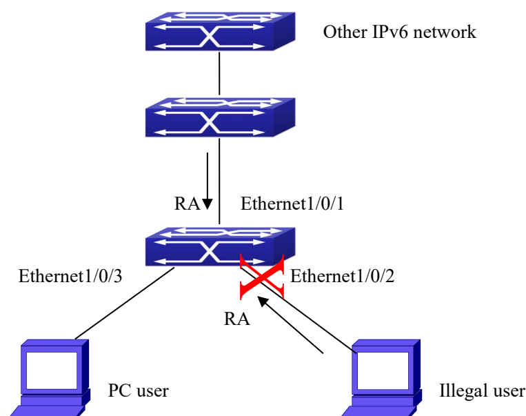
Figure 10-7 IPv6 Security RA sketch map
