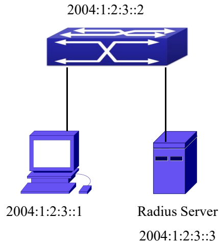
Figure 5-22 The Topology of IPv6 RADIUS configuration
