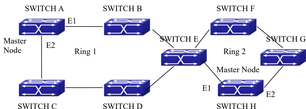
Figure 6-7 MRPP Sketch Map
