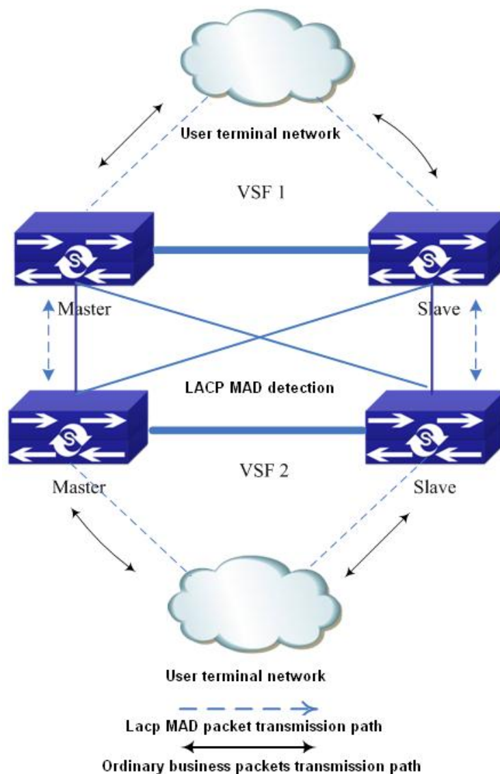
Figure 9-9 lacp mad detection topology
