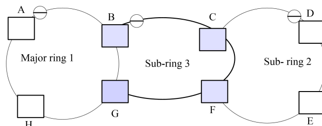
Figure 6- 19 the interconnection ring topology without virtual channel
