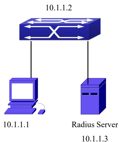
Figure 5- 21 The Topology of IEEE802.1x configuration
