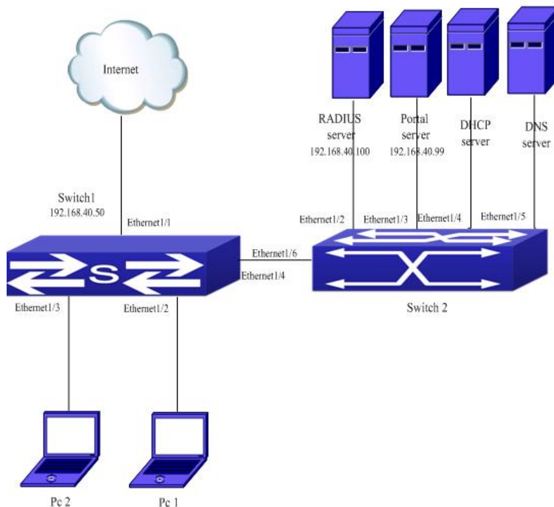
/Figure 5-26 authentication function configuration
