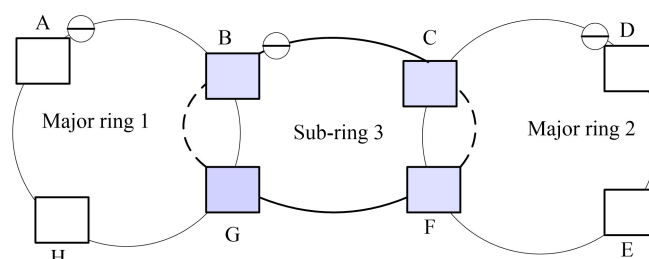
Figure 6- 18 the interconnection ring topology with virtual channel
