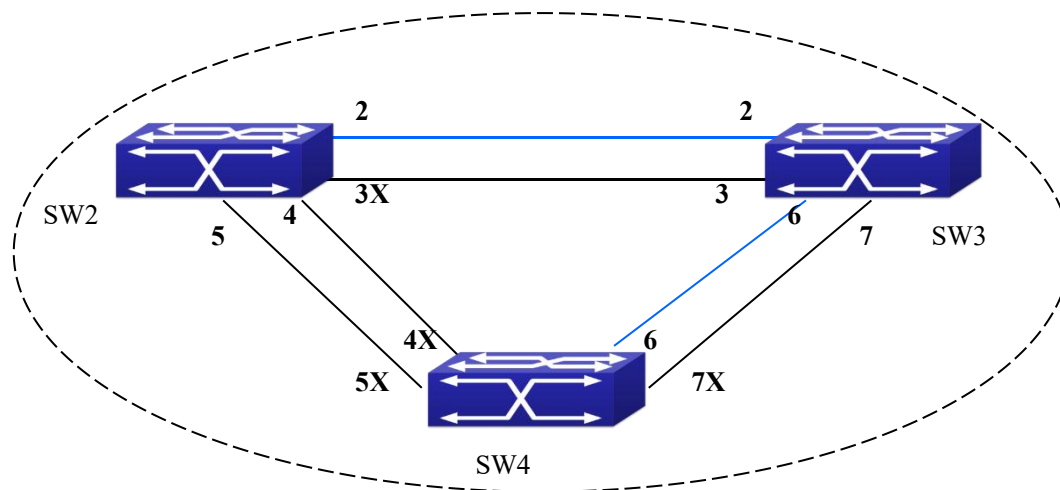
Figure 6-4 The Topology Of the Instance 3 after the MSTP Calculation
