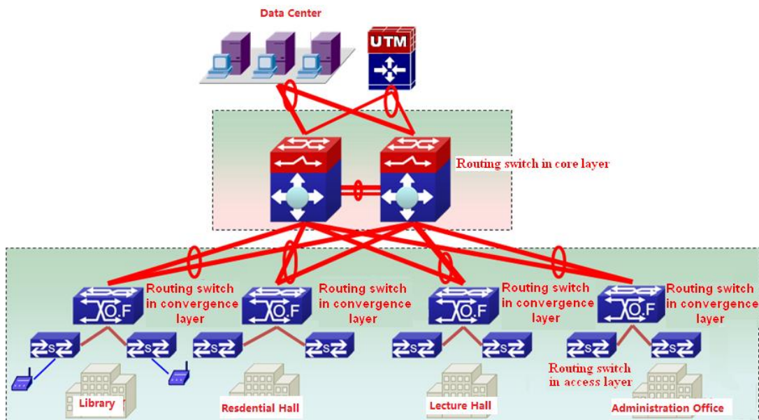
Figure 9-6 application of VSF in the campus data center
