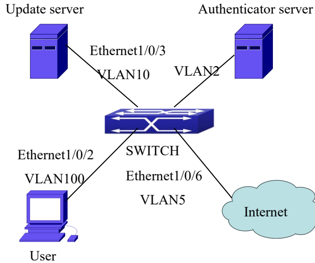
Figure 5-13 The Network Topology of Guest VLAN
