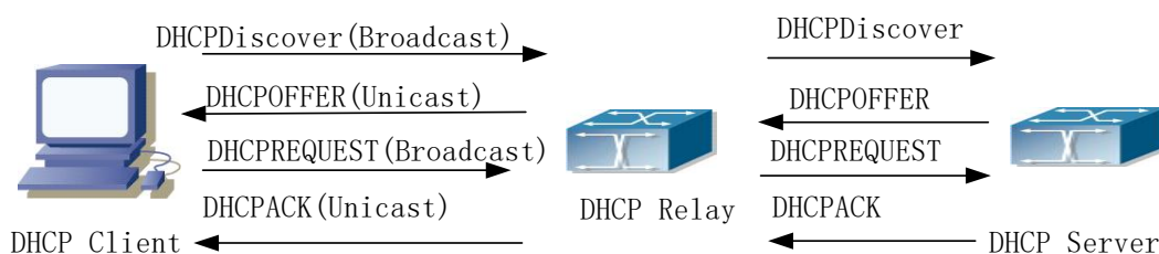
/ Figure 3-5 DHCP relay
