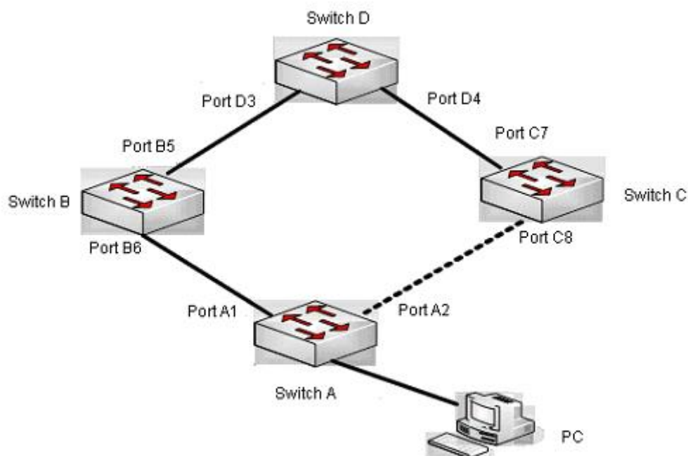
Figure 6-13 ULSM using scene
