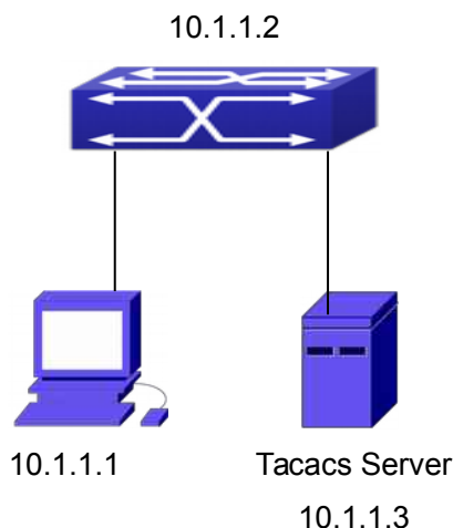
Fig 8-1 TACACS Configuration
