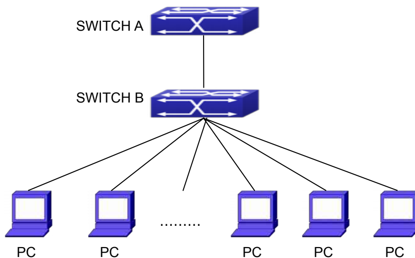
Fig 5-1 The Number Limitation of MAC and IP in Port, VLAN Typical Configuration
