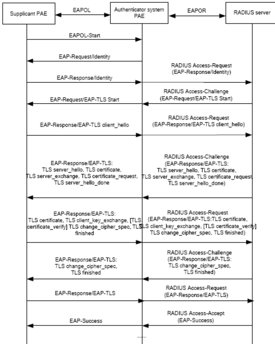
Fig 4-10 the Authentication Flow of 802.1x EAP-TLS
