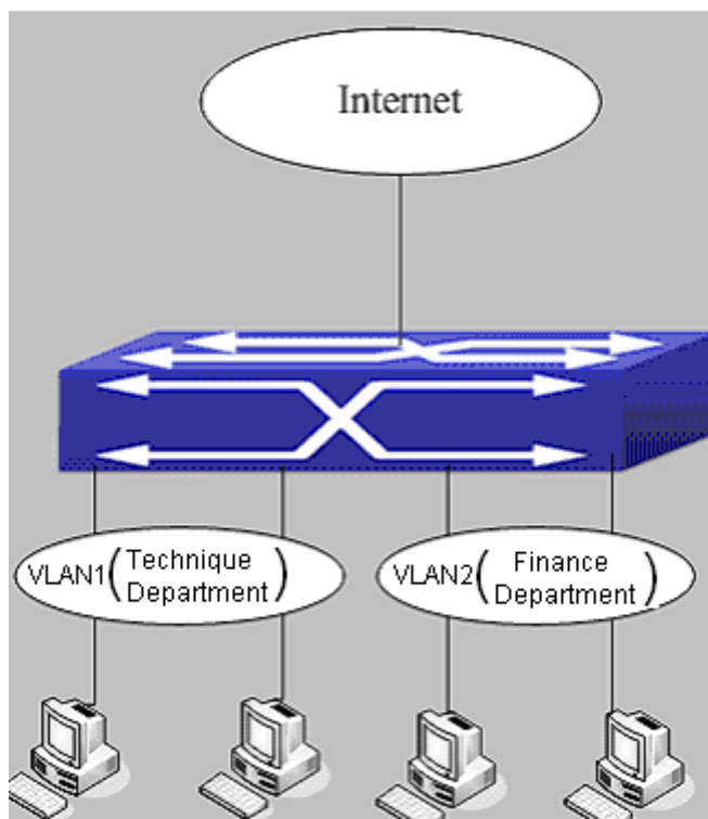
Fig 15-1 VLAN-ACL configuration example
