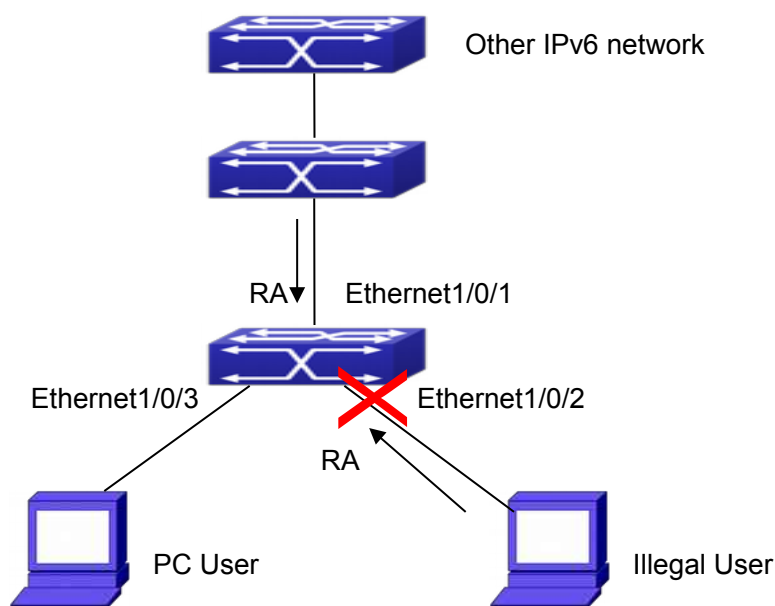
Fig 11-1 IPv6 Security RA sketch map
