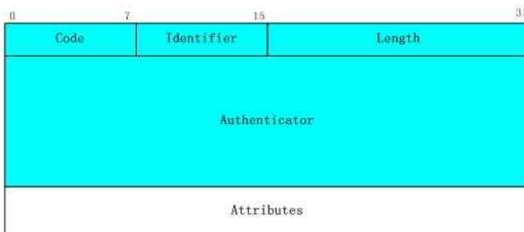
Fig 9-1 Message structure for RADIUS
