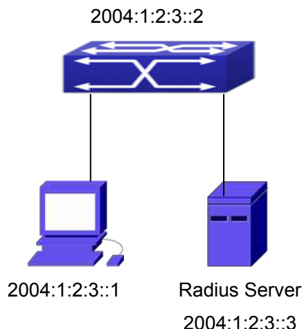
Fig 9-3 The Topology of IPv6 Radius configuration
