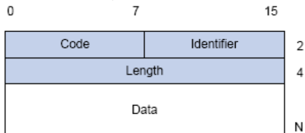
Fig 4-4 the Format of EAP Data Packets
