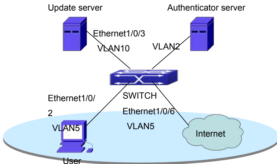
Fig 4-15 User Being Online, VLAN Being Offline
