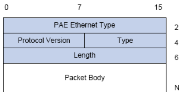
Fig 4-3 the Format of EAPOL Data Packet
