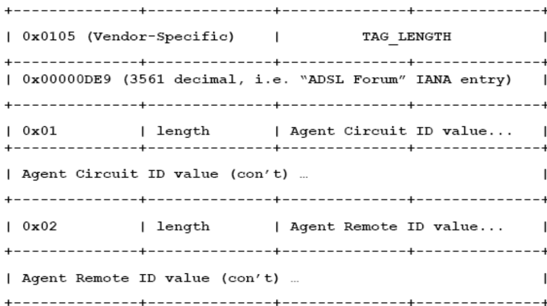
Fig 13-2 PPPoE IA - vendor tag (4 bytes in each row)
