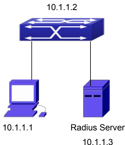
Fig 4-16 IEEE 802.1x Configuration Example Topology
