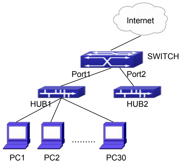
Fig 6-1 a typical configuration example of AM function
