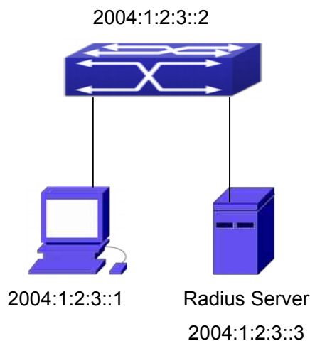
Fig 4-17 IPv6 Radius
