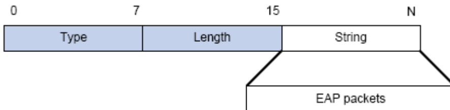
Fig 4-6 the Encapsulation of EAP-Message Attribute
