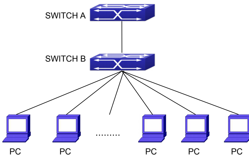
Fig 4-1 The Number Limitation of MAC and IP in Port, VLAN Typical Configuration
