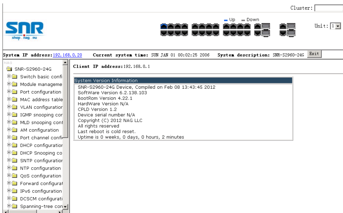
Fig 1-11 Main Web Configuration Interface
