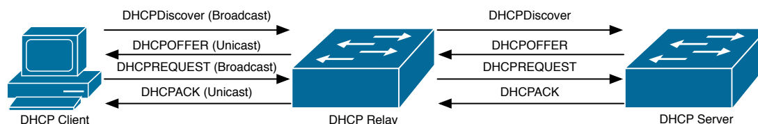
Figure 27.2: DHCP relay
