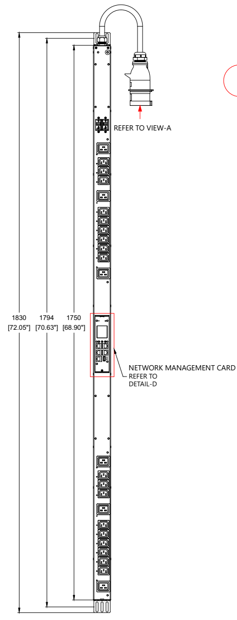
FRONT VIEW
