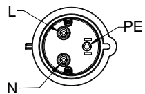
DETAIL A IEC309 32A, L+N+PE PLUG ENLARGED VIEW
