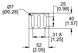
DETAIL C UNIVERSAL MOUNTING BRACKET ENLARGED VIEW
