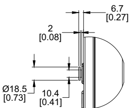
DETAIL B PEG TOOLLESS MOUNTING ENLARGED VIEW
