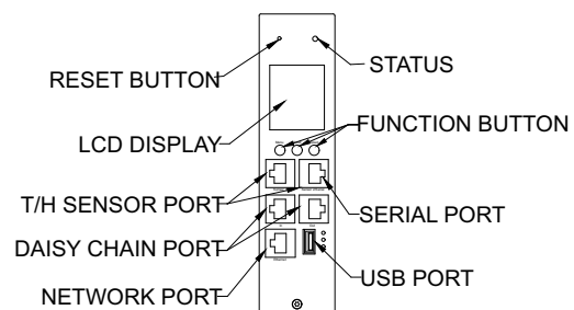
DETAIL D NETWORK MANAGEMENT CARD ENLARGED VIEW
