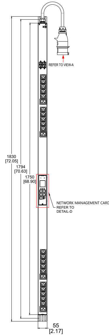
FRONT VIEW
