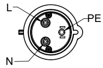
DETAIL A IEC309 32A, L+N+PE PLUG ENLARGED VIEW
