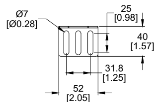
DETAIL C UNIVERSAL MOUNTING BRACKET ENLARGED VIEW
