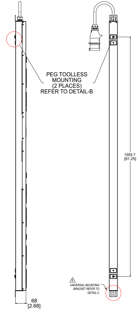
LEFT SIDE VIEW
