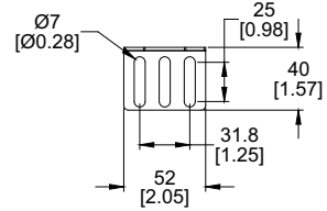
DETAIL C UNIVERSAL MOUNTING BRACKET ENLARGED VIEW
