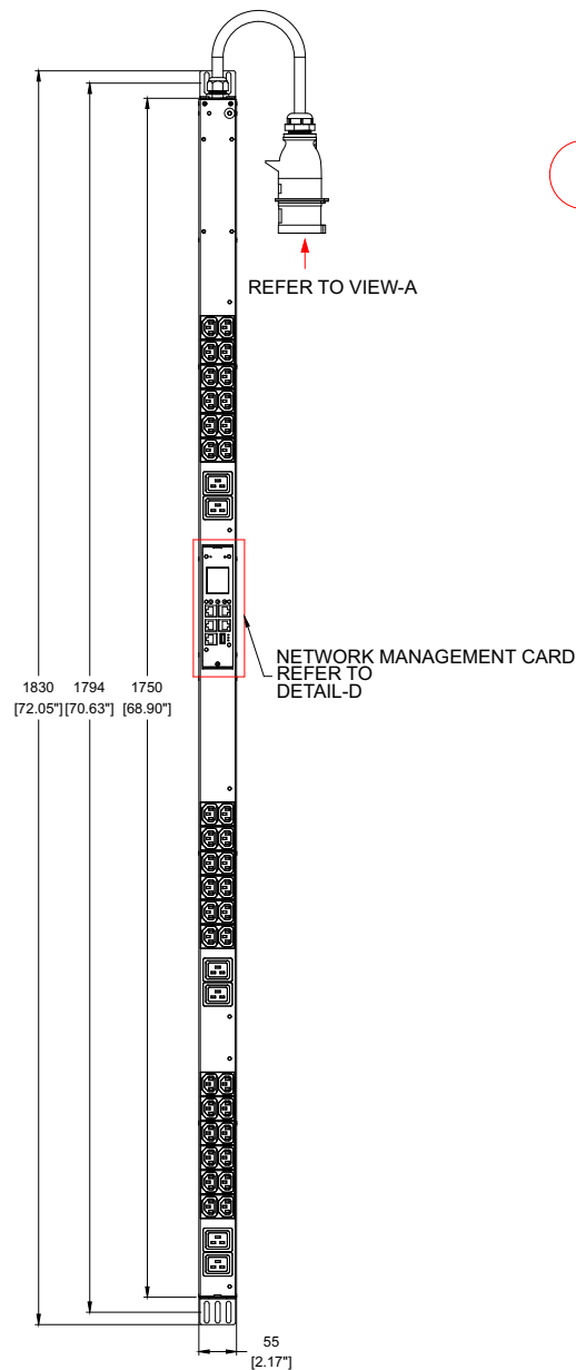
FRONT VIEW
