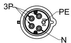
VIEW A IEC 309 16A 3P+N+PE PLUG ENLARGED VIEW
