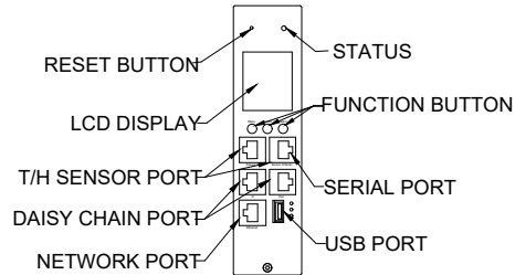
DETAIL D NETWORK MANAGEMENT CARD ENLARGED VIEW
