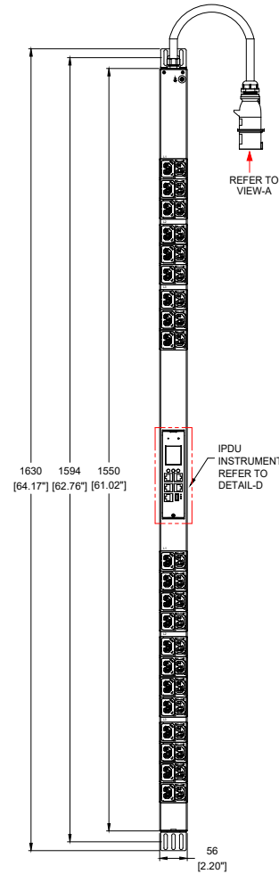
FRONT VIEW
