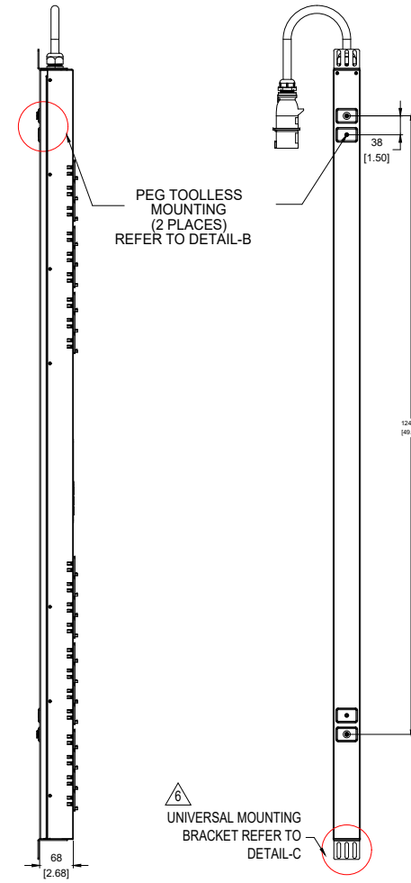
REAR VIEW
