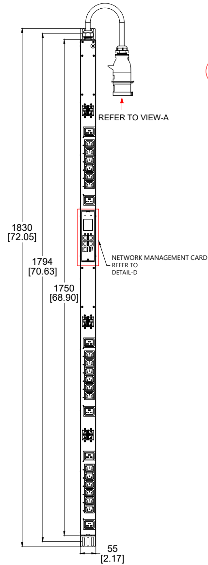
FRONT VIEW
