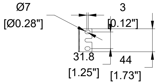
DETAIL A UNIVERSAL MOUNTING BRACKET ENLARGED VIEW
