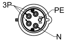
VIEW A IEC 309 16A 3P+N+PE PLUG ENLARGED VIEW
