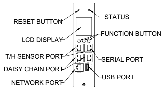
DETAIL C NETWORK MANAGEMENT CARD ENLARGED VIEW
