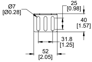
DETAIL B UNIVERSAL MOUNTING BRACKET ENLARGED VIEW
