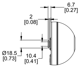
DETAIL A PEG TOOLLESS MOUNTING ENLARGED VIEW
