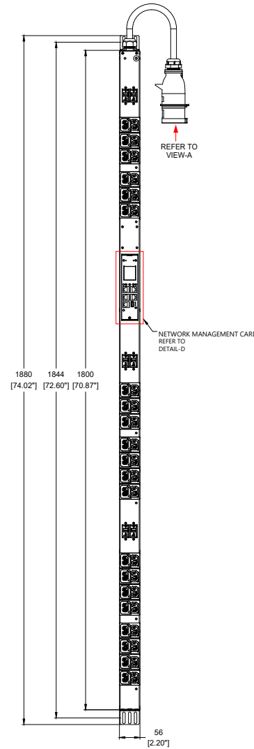
FRONT VIEW
