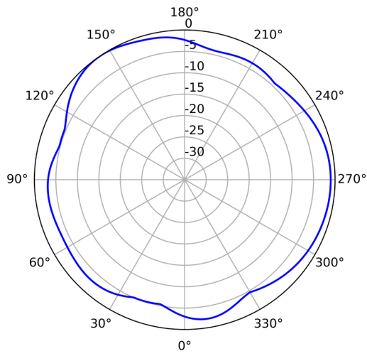
2.4GHz (Horizontal)
