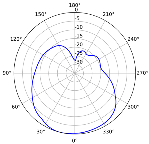
2.4GHz (Horizontal)
