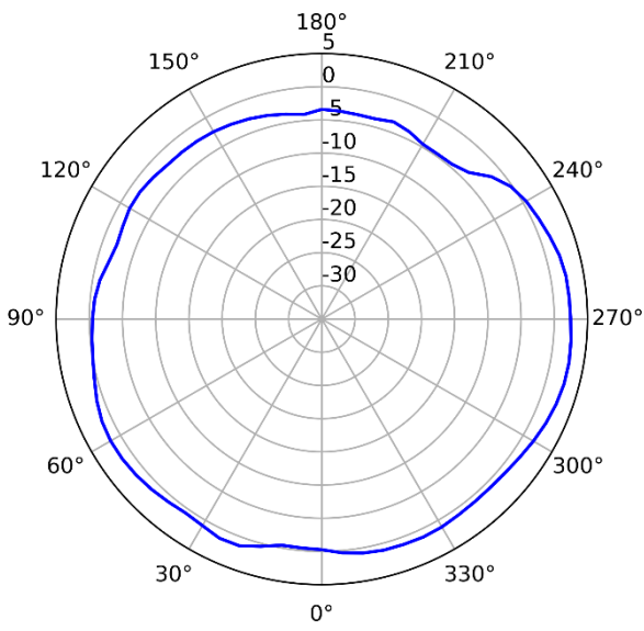
2.4GHz (Horizontal)
