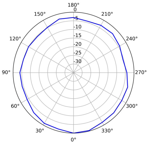
2.4GHz (Horizontal)
