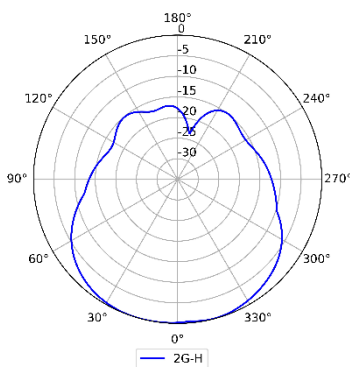
2.4GHz (Horizontal)
