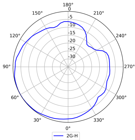
2.4GHz (Horizontal)
