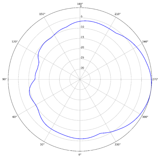
2.4GHz (Horizontal)
