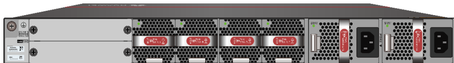
Figure 4-3 HiSecEngine USG6636F/USG6656F/USG6686F
